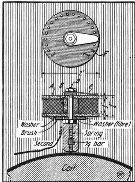
Loading Coil Mounted on Tuner Slider.
