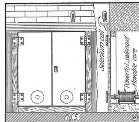
Fig. 5. Two Schemes for Opening and Closing Window Shutters at Sunrise and Sunset by a Selenium Cell.
