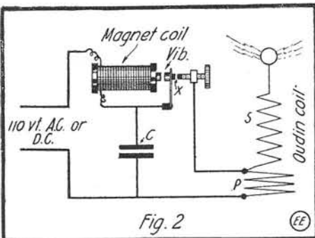
Fig. 2. Collins-Sanchez High Frequency Generating Circuit.
