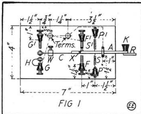
Fig. 1. Assembled Automatic Telegraph Key.
