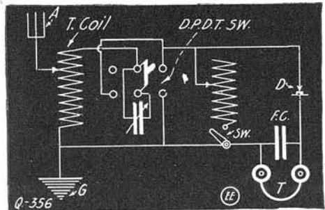
Wireless Receiving Tuning Diagram.
