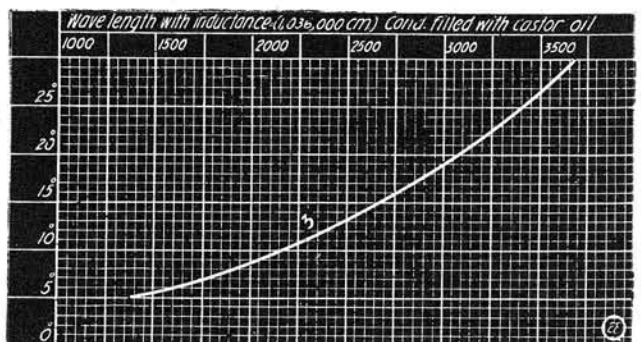
Fig. 9. Wave Length Inductance and Capacity Curves for Use With Wave Meter.
