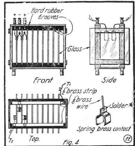
Fig. 4. Constructional Details of 12,000-Volt Glass Plate Condenser.
