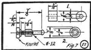
Fig. 7. Details of Binding Posts.
