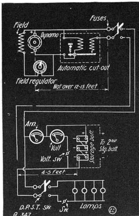
Wiring Diagram for Storage Battery Lighting Plants.
