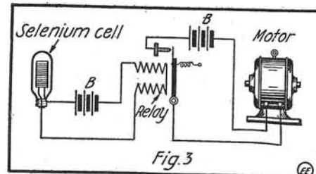
Fig. 3. Standard Connections for Selenium Cell and Relay.
