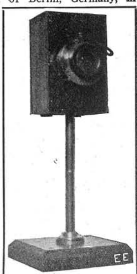
Fig. 10. Special Selenium Cell Device for Timing Photographic Shutters.
