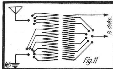
Fig. 11. Hook-Up for Coupler.
