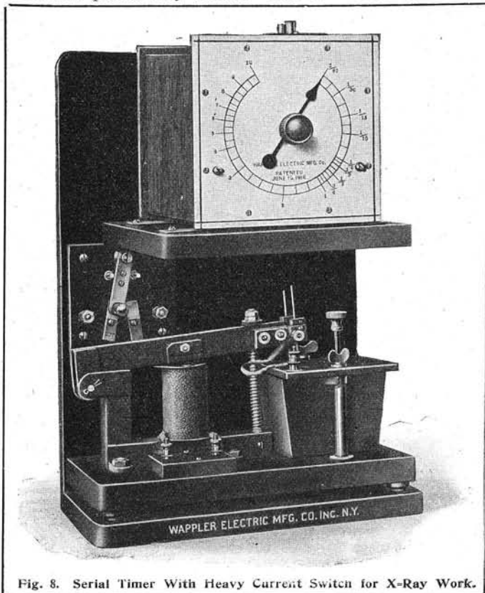
Fig. 8. Serial Timer With Heavy Current Switch for X-Ray Work.
