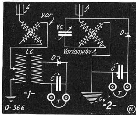
Variometer Hook-Ups.
