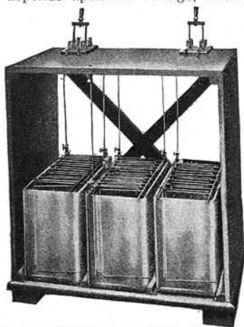
Fig. 2. Chemical Rectifier Capable of Handling Several Kilowatts.
