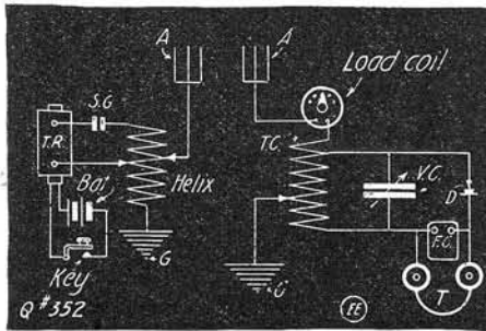
Radio Transmitting and Receiving Hook-ups.
