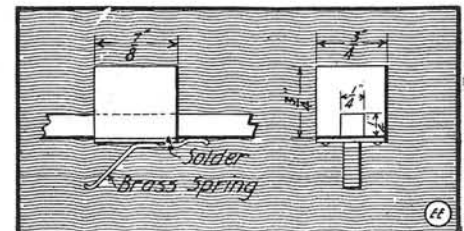
Tuning Coil Slider Made from Wood.
