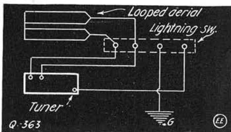
Looped Aerial Lightning Switch.
