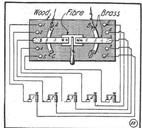
Unique Detector Switch.
