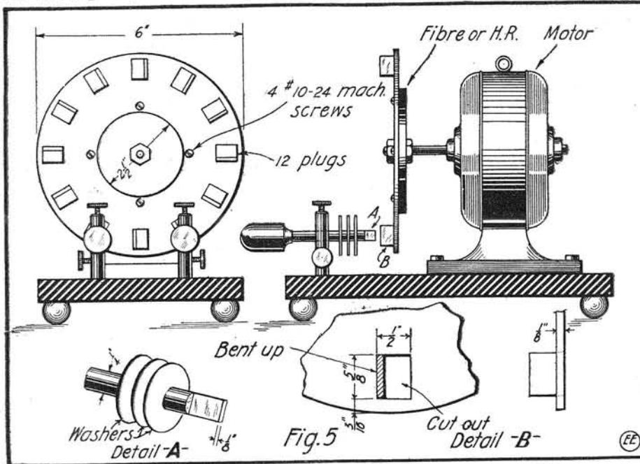
Fig. 5. Details of Rotary Spark Gap for 1/2-Kw. High Frequency Coil.
