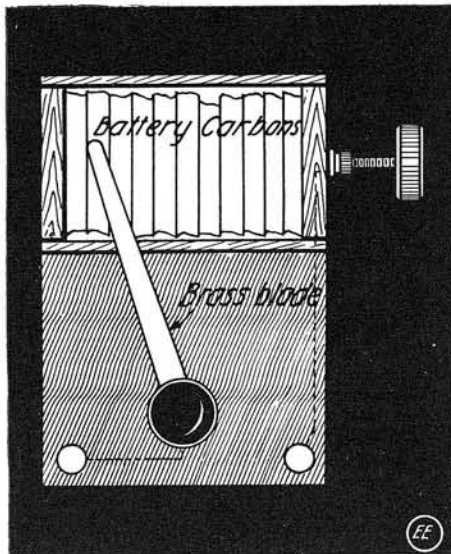
Old Battery Carbons Form Useful Rheostat.
