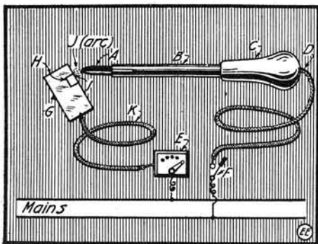
Arc Type Electric Soldering Iron.
