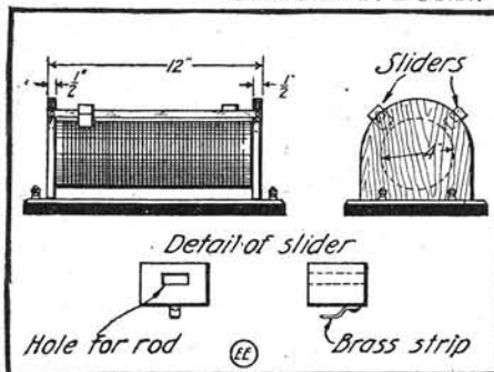
A Home-Made Tuning Coil.
