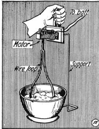
Home-Made Electric Egg-Beater.
