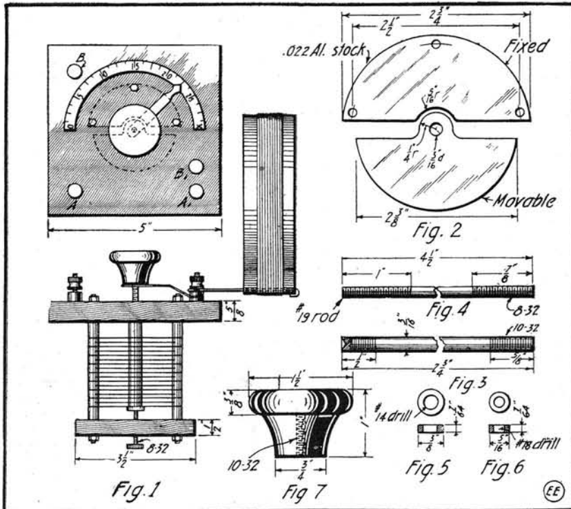
Details of Wave Meter Condenser and Inductances.
