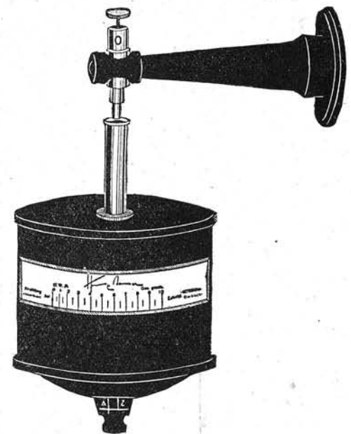
Fig. 5. Electro-Static Type of X-Ray Penetrometer.
