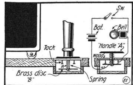
Removing Chair From Spring Switch Gives Alarm.
