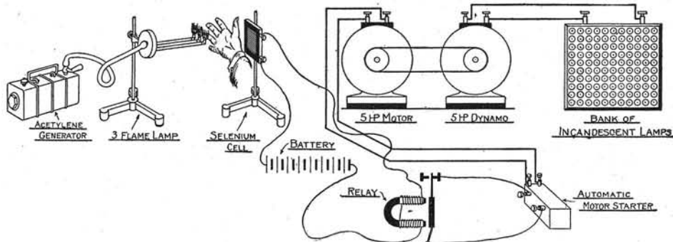
Fig. 11. Arrangement as Used by Wm. J. Hammer for Controlling a 5 Horsepower Motor by a Wave of the Hand.
