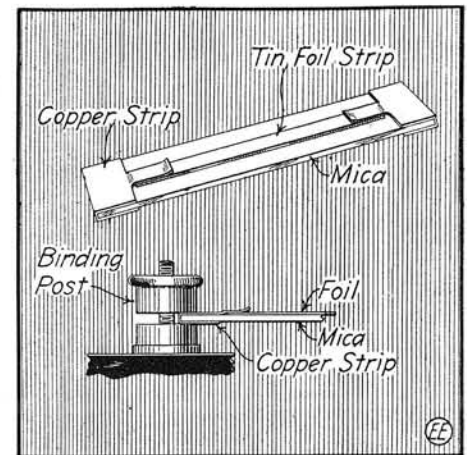
Battery Fuses Made from Tin-Foil and Mica.
