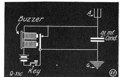
Buzzer Used for Transmitting Radio Signals.
