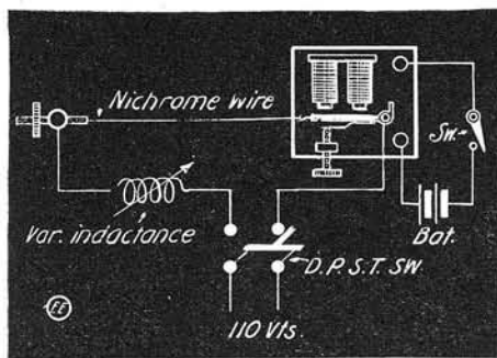
Making Mechanical Waves on Wire Visible.
