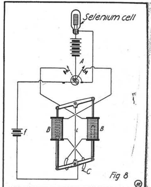
Fig. 8. Circuits of Gas Lighted Buoy Controlled by Sun's Rays Affecting Selenium Cell.
