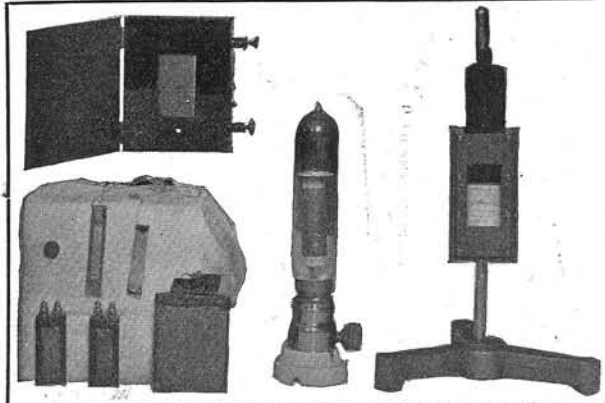
Fig. 1. Several Specimens of Successful Selenium Cells.
