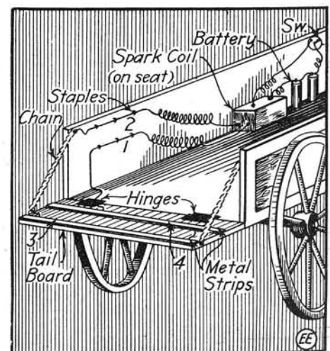
Spark Coil to Keep Children Off Wagon Tail-Boards.
