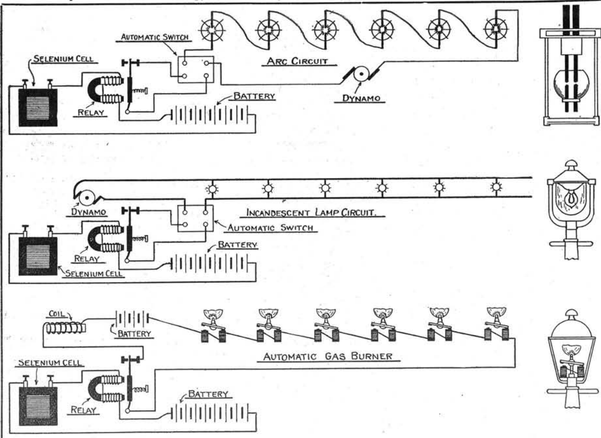
Fig. 4. Scheme for Turning On and Off Street Lights by Means of Selenium Cells, as Devised by William J. Hammer.
