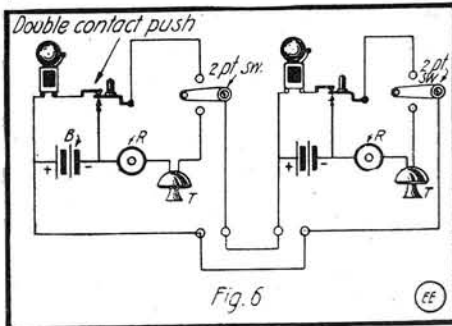
Fig. 6. Connections of Dictaphone Set.
