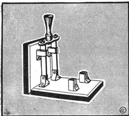
Aerial Switch Composed of 2 D.P.S.T. Knife Switches.
