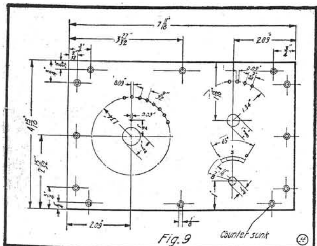
Fig. 9. Switch Lay-Out for Inductive Coupler.
