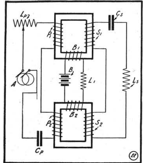
Frequency Changer, Using Transformers Specially Arranged.
